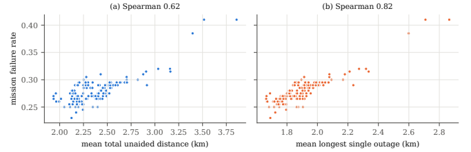
Fig. 2. Mission failure versus (a) mean total unaided distance and (b) mean longest outage, for 150 routes (Study A, no camera).
