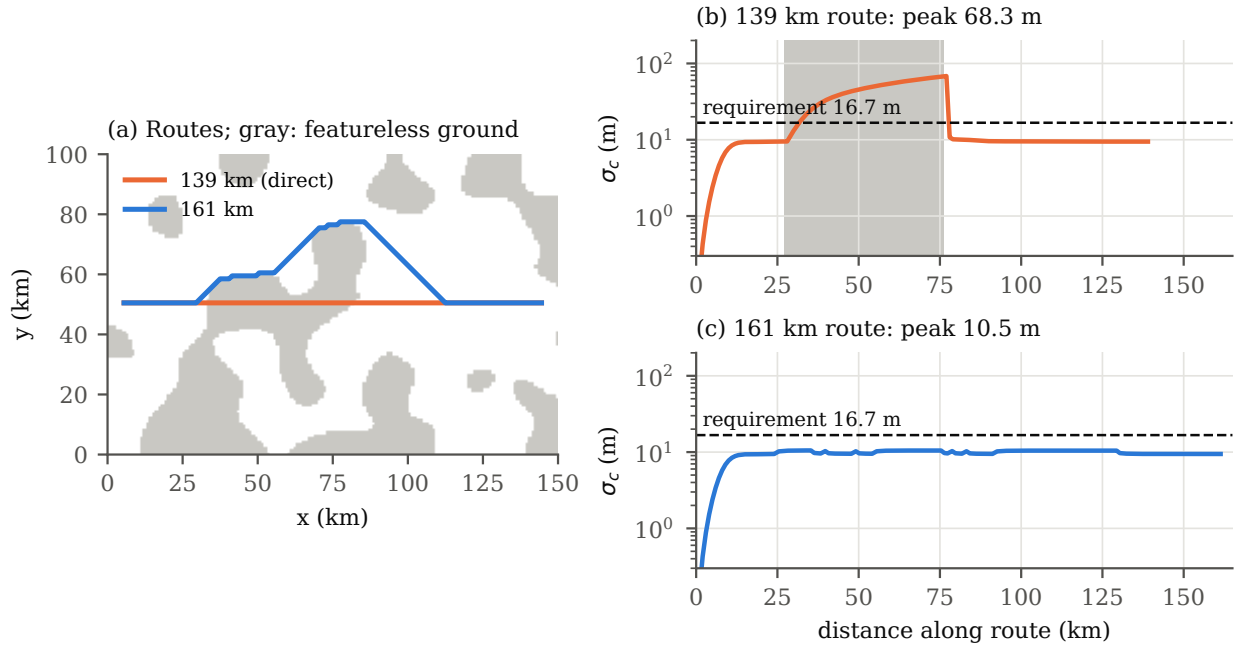
Fig. 6. Running example: the same architecture (1,000 LEO satellites, 7-element array, eLoran, thermal camera, navigation IMU) on two routes, on one test field where the satellite layer is lost and eLoran is in a regional outage. (a) The routes over the terrain; gray: featureless ground, where the camera gives no map fix. (b, c) Cross-track navigation uncertainty along each route; gray: featureless stretches; dashed: the requirement.
