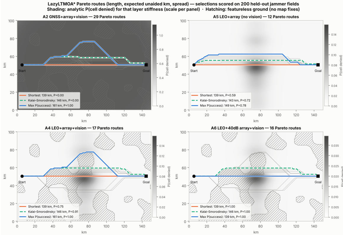
Fig. 3. Study A: Pareto routes (gray) for four user configurations, with the shortest, Kalai-Smorodinsky, and most reliable routes highlighted; shading is the analytic denial probability, hatching featureless ground. (Fronts computed without the endurance limit.)
