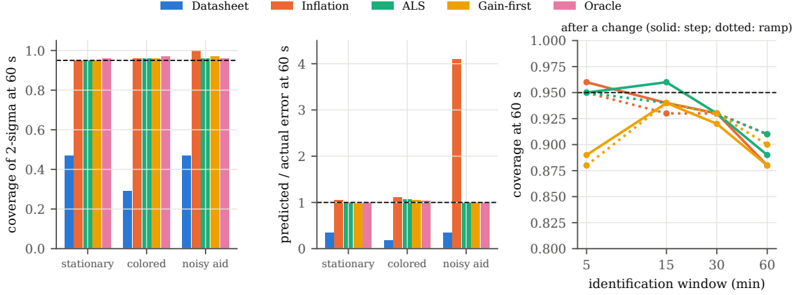
Fig. 1. Coasting-law estimators: coverage of the predicted 2\sigma envelope at 60 s (left) and ratio of predicted to actual error (middle) in three stationary scenarios; coverage versus identification window after a change of conditions (right).
