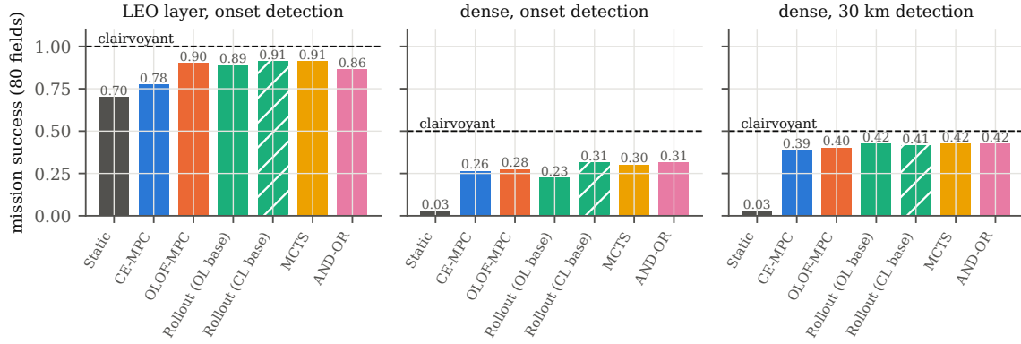
Fig. 4. Mission success by policy in three cases (80 fields); dashed: clairvoyant reference.
