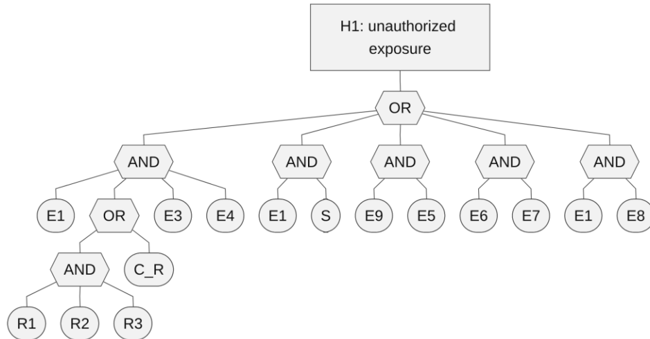
Figure 2. Fault tree for H1. The demand event E1 appears in three branches; four of the five branches are second-order.
